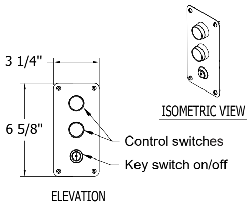
WALL MOUNTED
